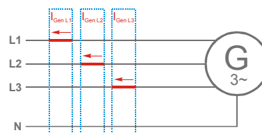
Figure 6-34: Current measuring - generator, L1 L2 L3
