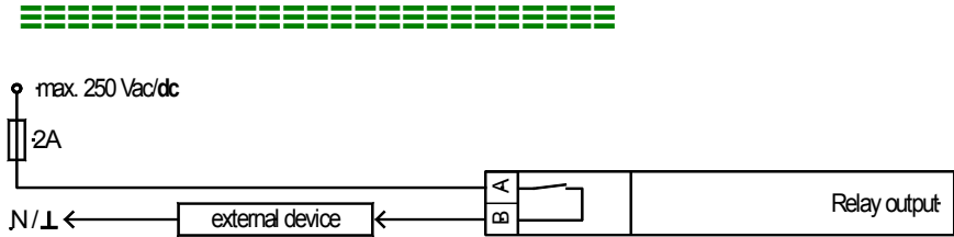
Figure 6-46: Relay outputs
