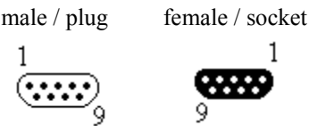
Figure 9-1: CAN bus pin assignment - D-SUB DE9 connector
