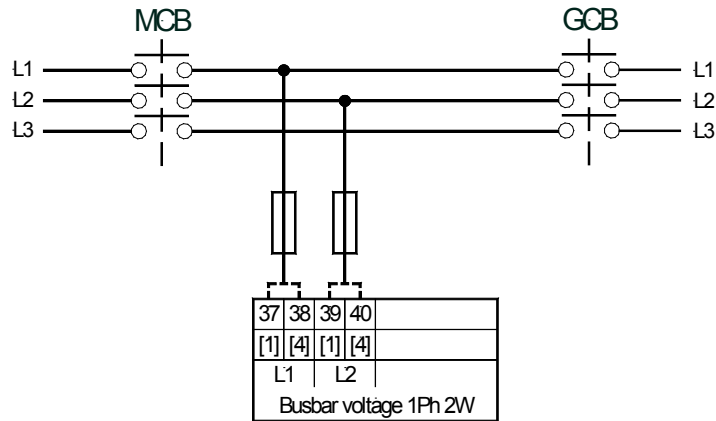
Figure 6-32: Voltage measuring - busbar measuring inputs, 1Ph 2W (phase-phase)
