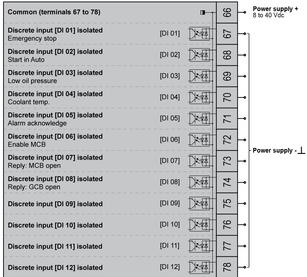
Figure 6-44: Discrete inputs - alarm/control input - negative signal
