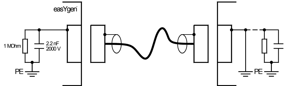
Figure 6-58: Interfaces - shielding
