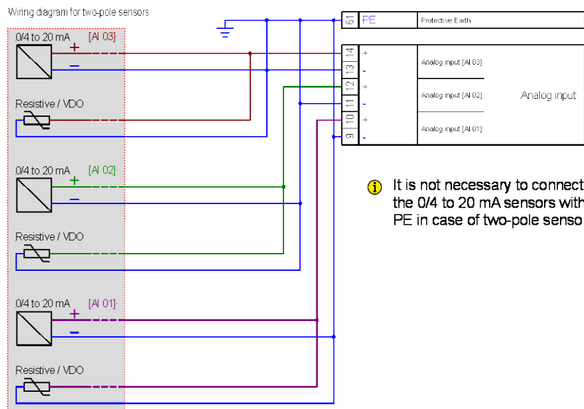
Figure 6-47: Analog inputs - wiring two-pole senders
