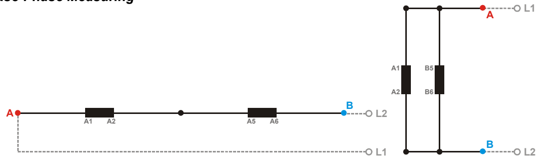
Figure 6-31: Voltage measuring - busbar PT windings, 1Ph 2W (phase-phase)
