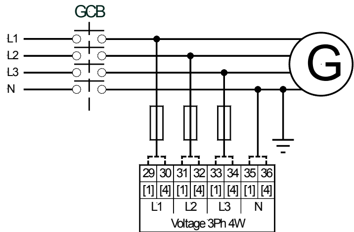
Figure 6-8: Voltage measuring - generator measuring inputs, 3Ph 4W
