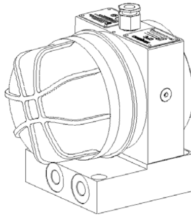
New CPC with I/H Adapter Block (existing hydraulic tubing left in place)
