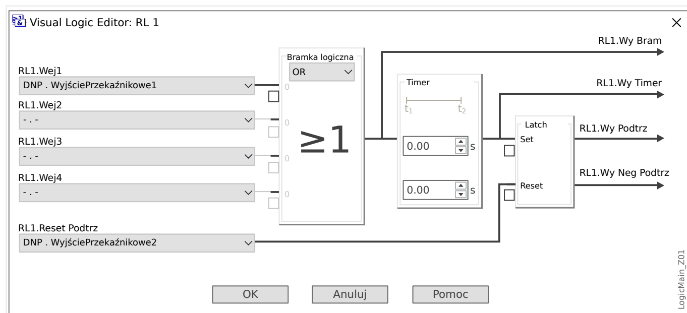
Rys. 59: Setting example from Smart view, to make a steady state signal from a DNP output signal.
