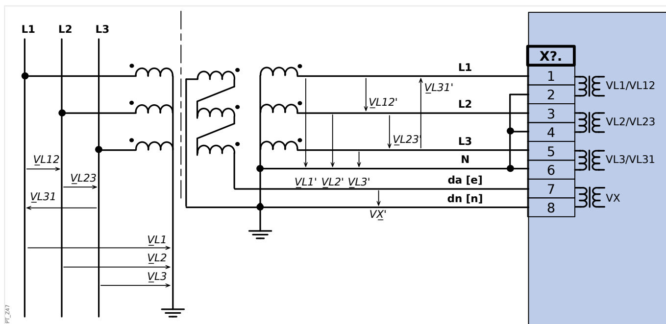
Fig. 35: VT Wye com conexão Broken Delt.
