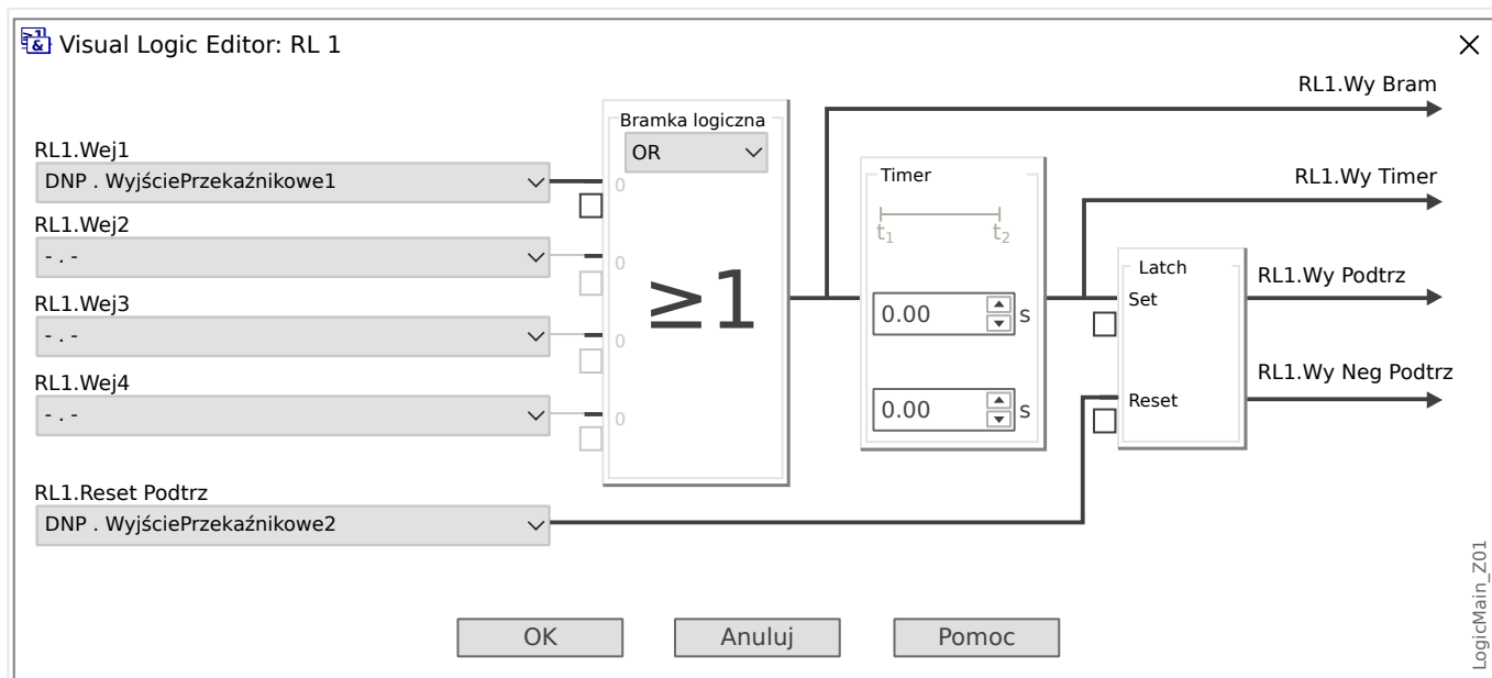
Rys. 55: Setting example from Smart view, to make a steady state signal from a DNP output signal.
